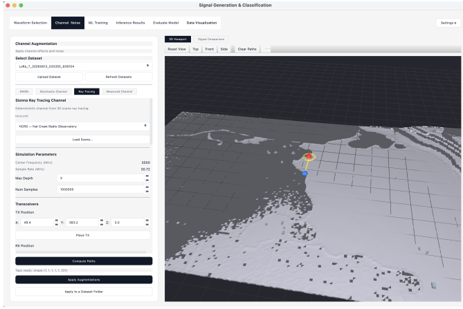
Fig. 2. Ray-tracing view with the imported HCRO scene. The transmitter and receiver were positioned by clicking directly on the rendered terrain, which ray-casts onto the scene surface, and the solver then returned the propagation paths and the channel taps for that pair. Any bundled or user-supplied scene loads into the same view.
