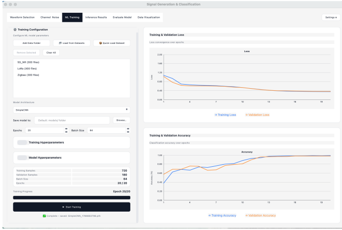
Fig. 3. Training view at the end of a run: the default compact 1-D CNN trained on the three-class measured-channel dataset, in which each example was convolved with a CMAT channel response drawn from the imported bank. Loss and accuracy are shown for the training and validation partitions.
