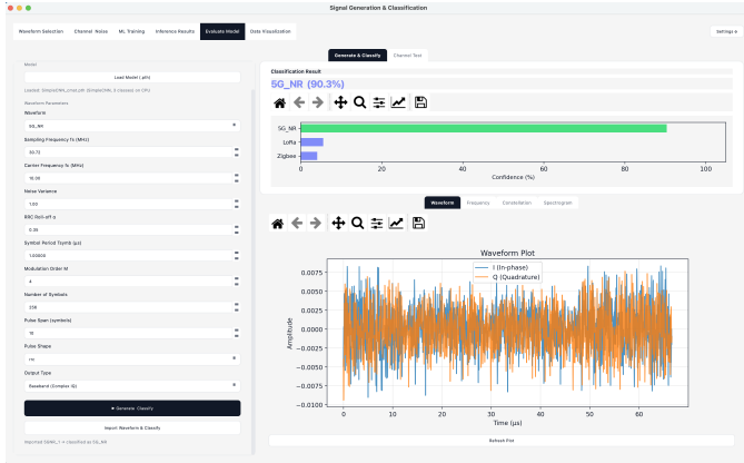
Fig. 4. Evaluation view scoring an imported recording. A 5G NR capture collected onsite at HCRO is loaded from disk and classified by the model of Fig. 3, which was trained only on measured-channel-augmented synthetic data; the view reports the predicted class with its confidence beside the signal in time and frequency.
